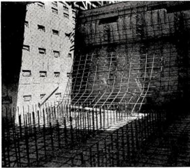
Inside the blast pit of one of the launcher buildings under construction.
